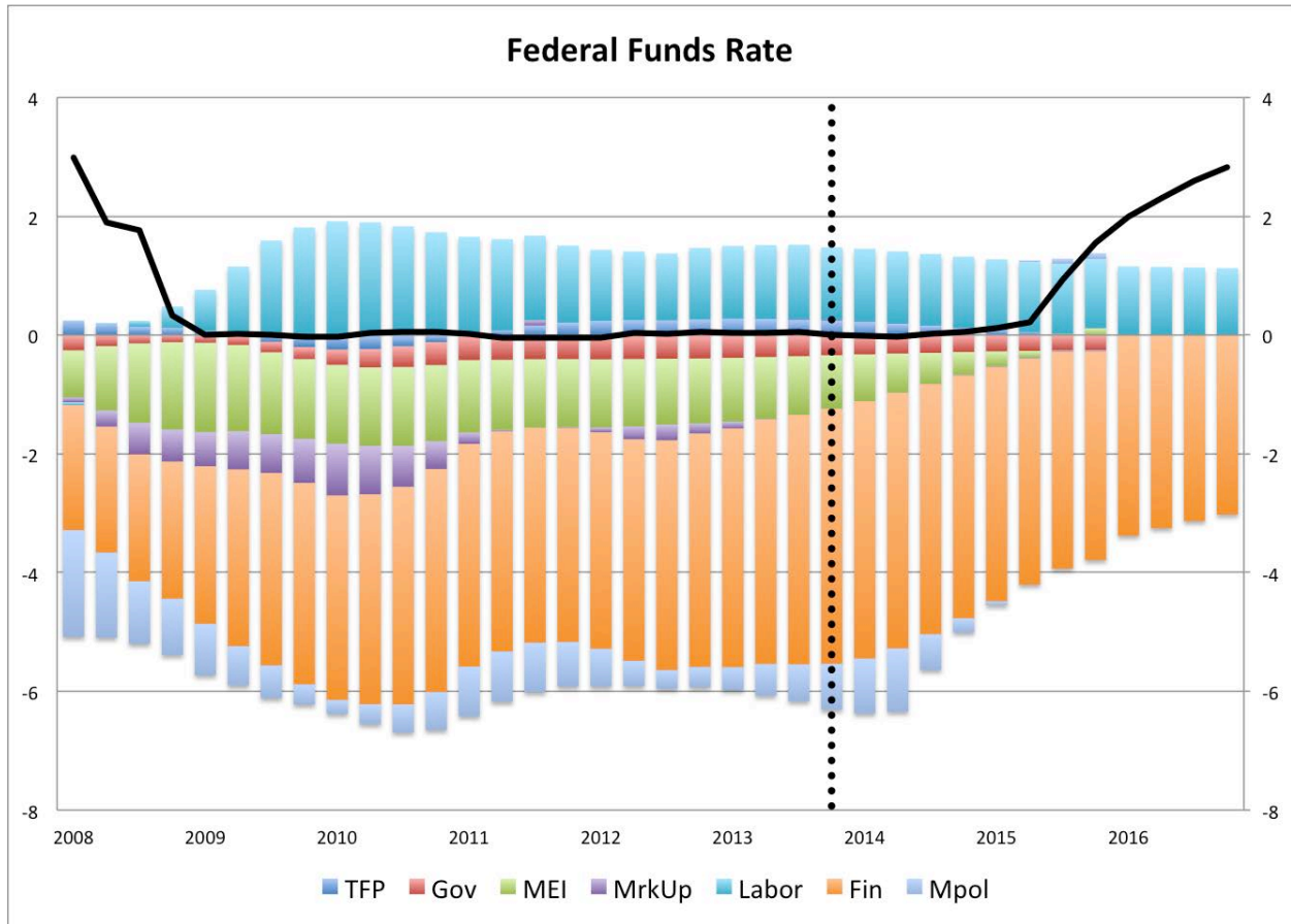
Figure 2c Conditional Forecast
