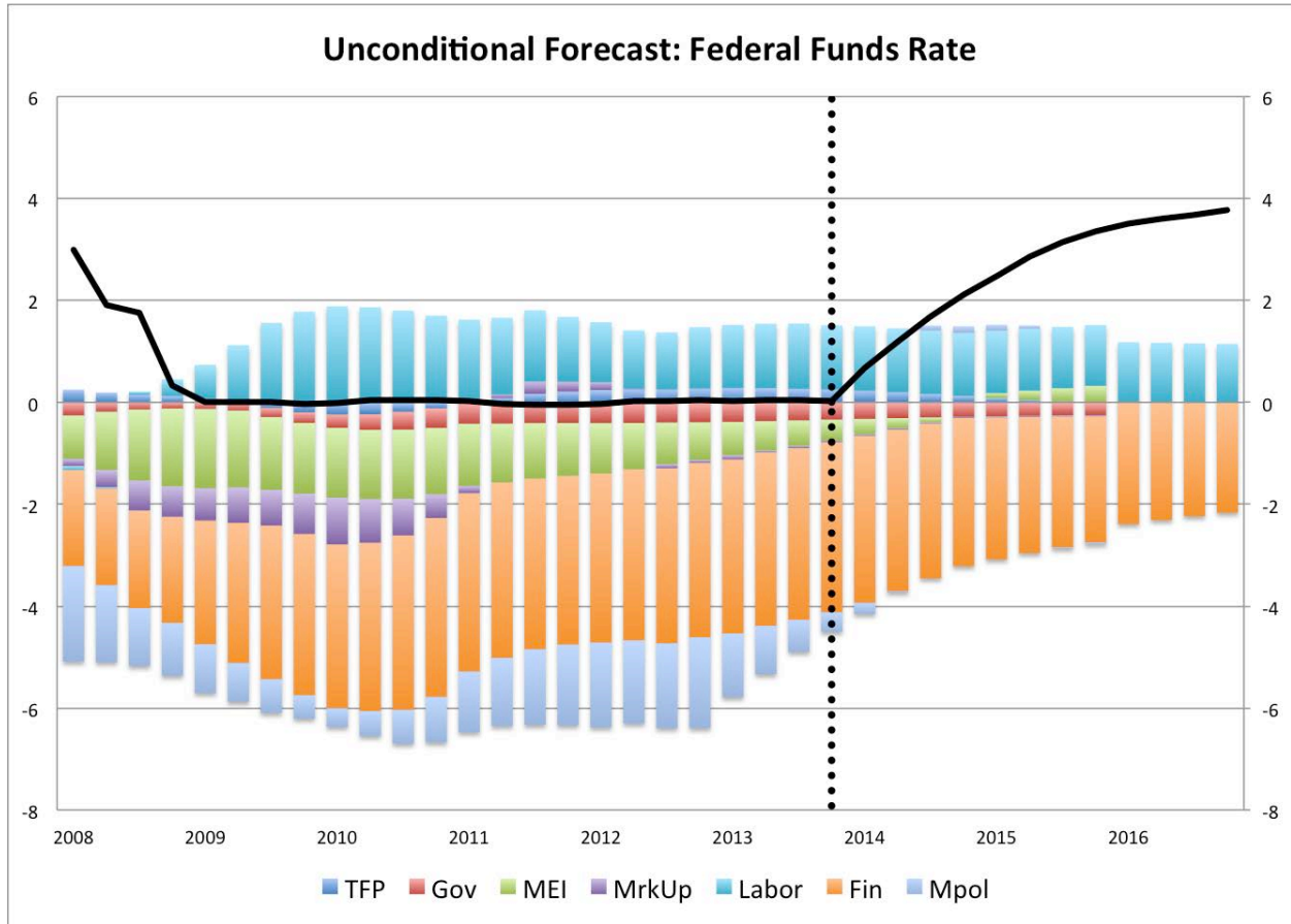
Figure 4c Unconditional Forecast
