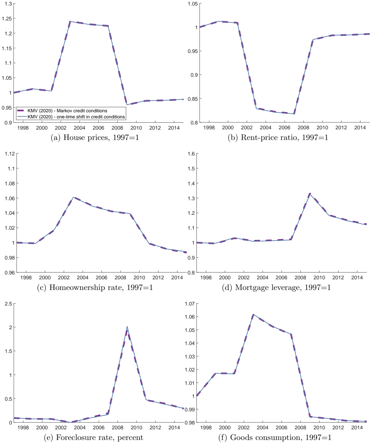
Figure 17: Housing boom impulse responses under exogenous beliefs, 1997=1.
