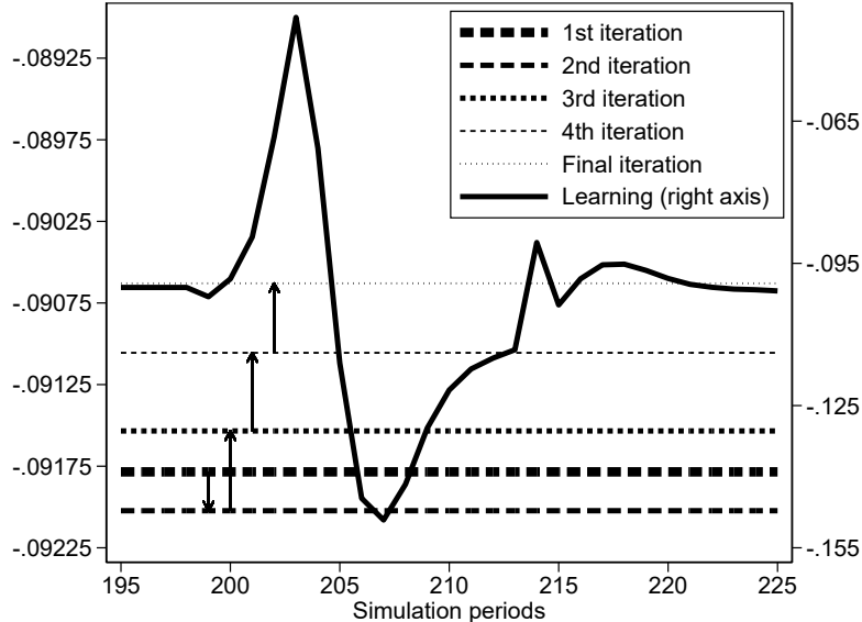
Figure 1: House price forecast coefficient a_{Z_{low_t}, Z'_{low}}^0 solved for as a fixed point or sequentially or under learning, which starts in period 200. The spikes in the coefficients under learning (solid thick line) are periods where the economy changes aggregate states. The coefficients eventually return to near their ergodic distribution (pre 200 values) by about period 220.
