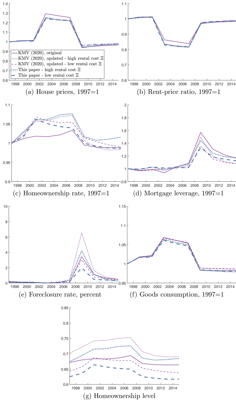
Figure 16: Housing boom impulse responses under exogenous beliefs, 1997=1.
